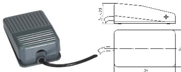
LJFS1-2(塑壳Plastic cover)
